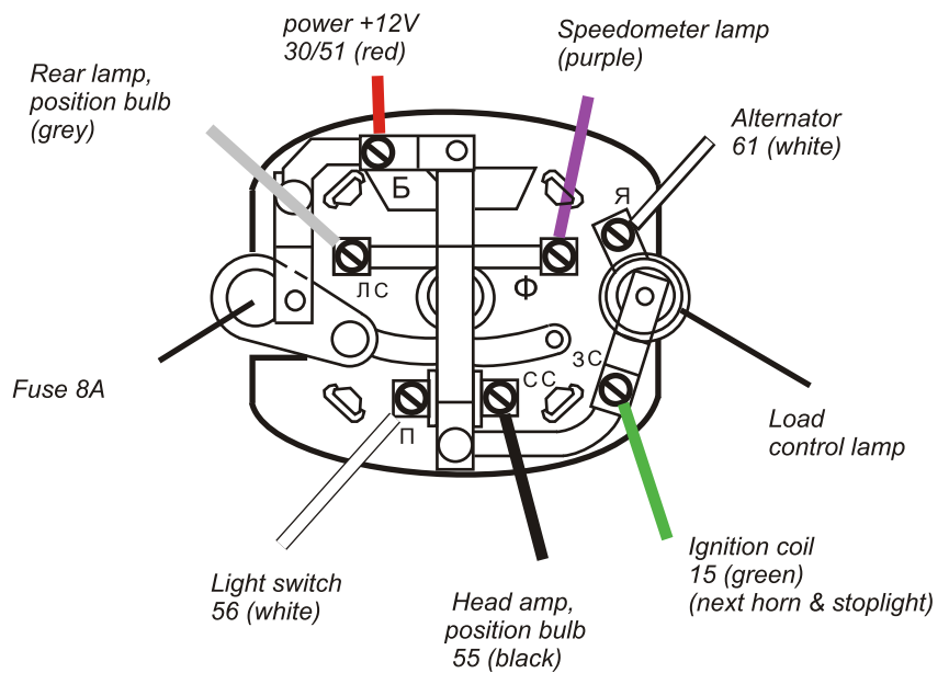
Fig. 5 Ignition switch diagram
